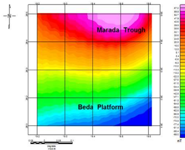
Figure 6: Total Magnetic Intensity Map
