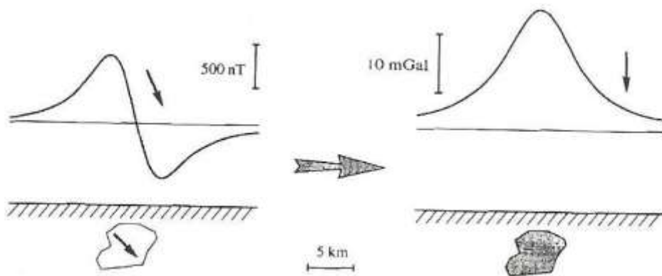
Figure 8: Magnetic anomaly and its pseudogravity transform (after Blakely 1995).
