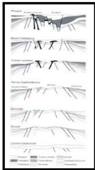
Figure 2. Structural development of sirt basin region lower Paleozoic to present after (Massa and delorte 1984.).
