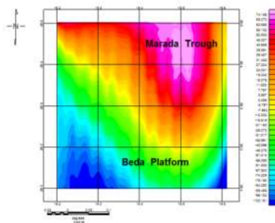
Figure 7: RTP map of study area.
