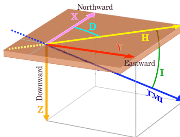
Figure 5: Elements of the magnetic field
