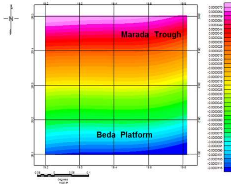
Figure 9: Pseudogravity map of study area
