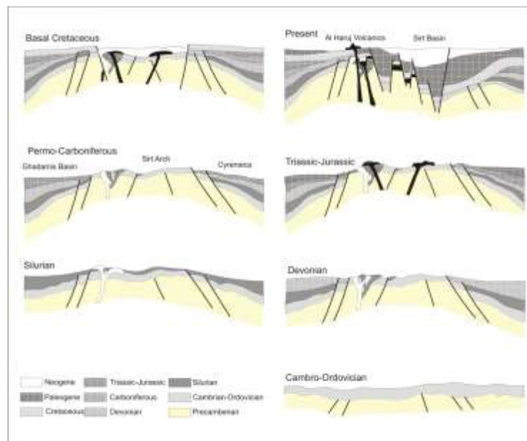
Figure 4: Structural development (E-W) of the Sirt Basin from the Lower Palaeozoic to the present time (Swei, 2010).
